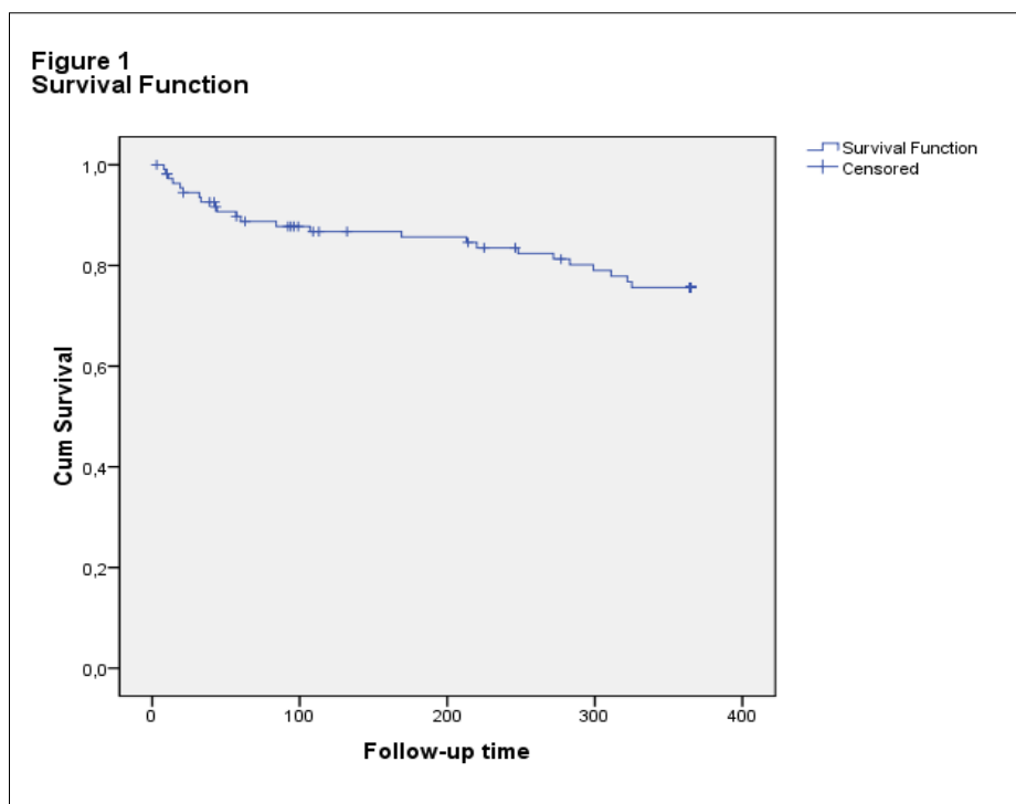
Figure 1: Survival Function
